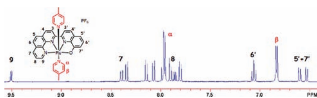
Figure 2. Downfield region of the 400 MHz ^1\text{H} NMR spectrum of [\text{Ru}(\mathbf{7b})(\text{pic})_2](\text{PF}_6) in \text{CD}_3\text{CN} .
