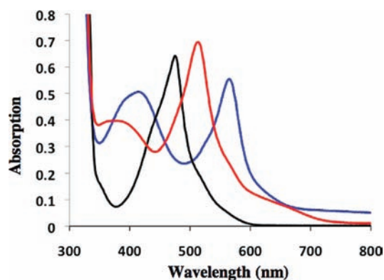
Figure 4. Long wavelength region of the electronic absorption spectra of [Ru(tpy) 2 ](PF 6 ) 2 (black), [Ru(tpy)( 6b )](PF 6 ) (red), and [Ru( 6b ) 2 ](PF 6 ) (blue).
