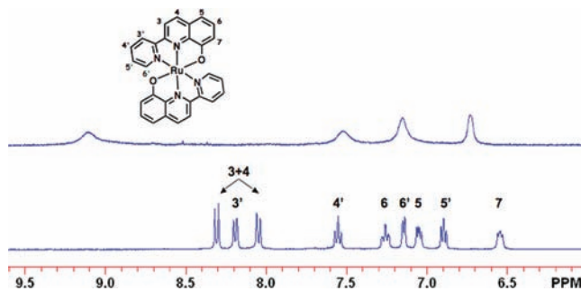
Figure 1. Downfield region of the 400 MHz ^1\text{H} NMR spectrum in \text{CD}_3\text{OD} of [\text{Ru}(\mathbf{6b})_2]^{2+} before (top) and [\text{Ru}(\mathbf{6b})_2] after (bottom) the addition of ascorbic acid.
